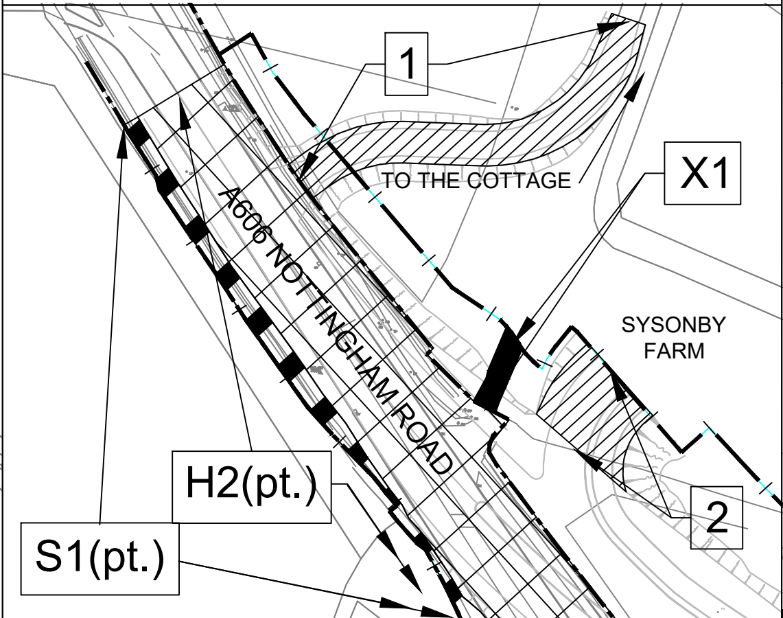
INSET 1 - New Private Means of Access to The Cottage & Sysonby Farm Scale 1-750 @ A1
