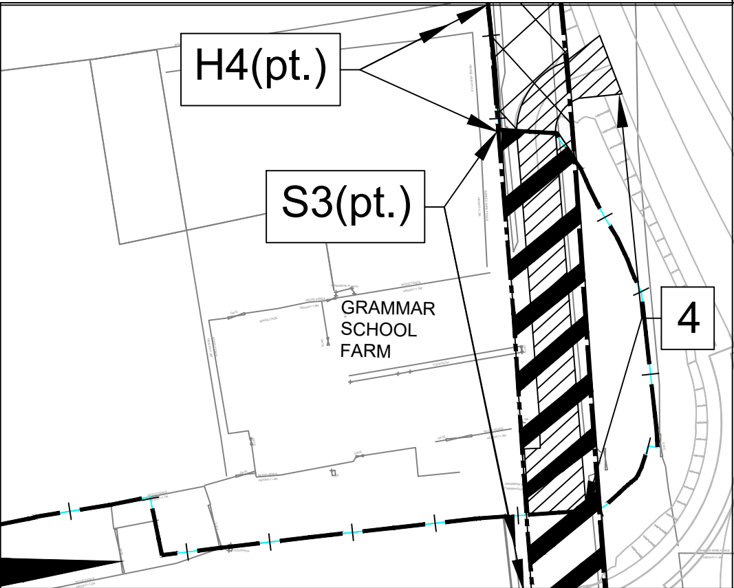
INSET 3 - Access to Grammar School Farm Scale 1-750 @ A1
